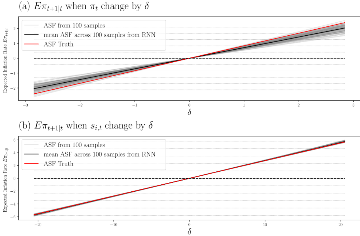
Figure 11: Estimated Average Structural Function from random samples using RNN. Function depicts change of expected variable in response to corresponding signal change by \delta . Panel (a): expected inflation as function of inflation signal \pi_t . Panel (b): expected inflation as function of private signal s_{i,t} . Red solid line is the actual ASF implied by linear Kalman Filter. Solid black line is the mean of estimated ASF from 100 random samples. Grey lines are estimated ASFs from each random sample.
