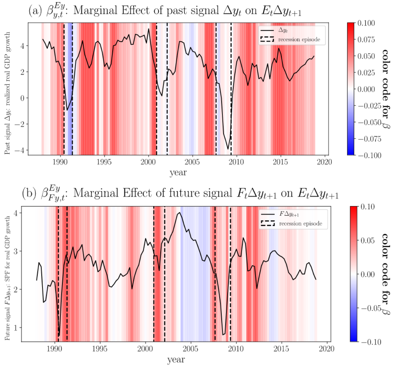
Figure 4: Color bars in panel (a): the marginal effects of real GDP growth signal \Delta y_t on expected economic condition next year E \Delta y_{t+1|t} . Panel (b): the marginal effects of professionals' forecasts about real GDP growth next year F \Delta y_{t+1|t} on expected economic condition. Red color: positive marginal effect; blue color: negative marginal effect. Black solid line: data on frequency of news about recession.
