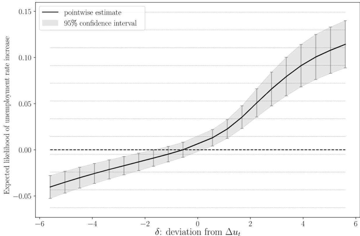
Figure 2: Average change of unemployment expectation E_t \Delta u_{t+1} , when unemployment signal \Delta u_t change by \delta . This is obtained by point-wise estimation of (12) at 20 different points of \delta , following the Double-Debiased Machine Learning approach from Chernozhukov et al. (2018), 95% confidence band is reported at each point-wise estimate. The estimate is depicted as solid black line, shaded area is implied 95% region.
