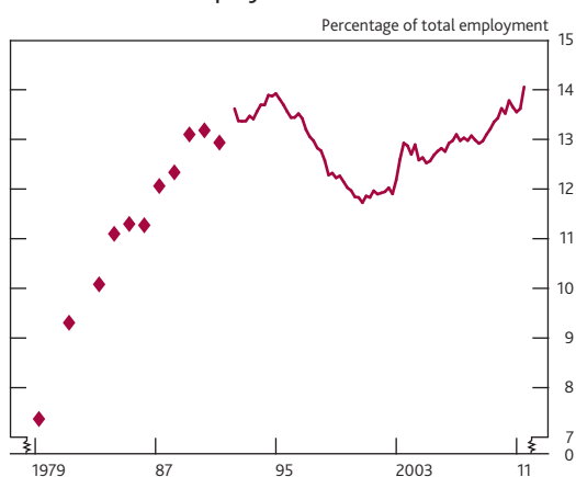
Chart 3.5 Self-employment (a)
