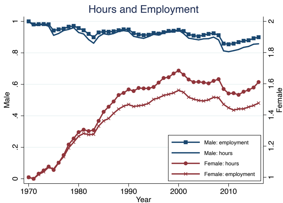
Figure 12: Employment Rates vs. Hours: Males and Females
