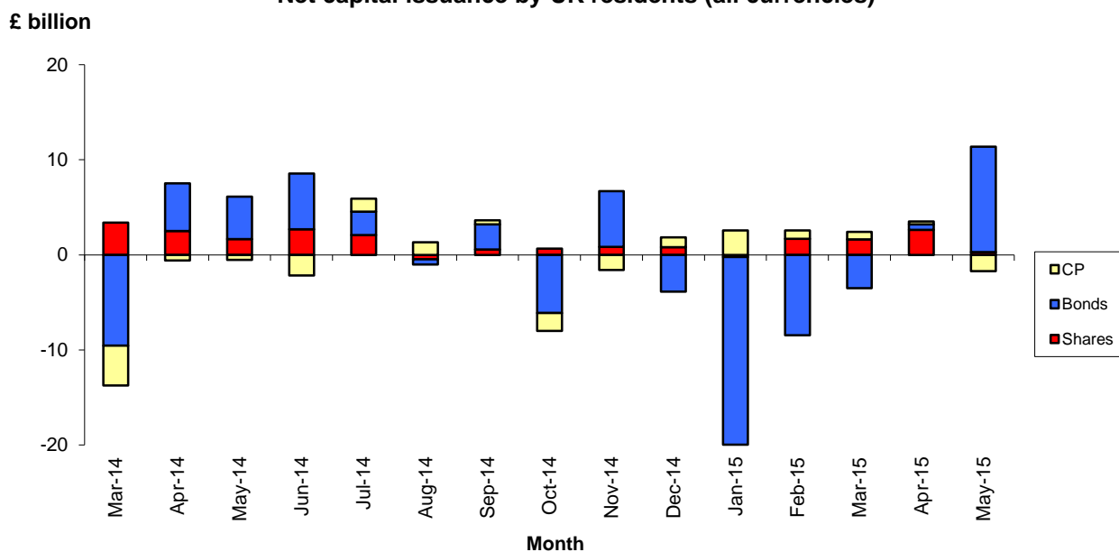
Net capital issuance by UK residents (all currencies)
