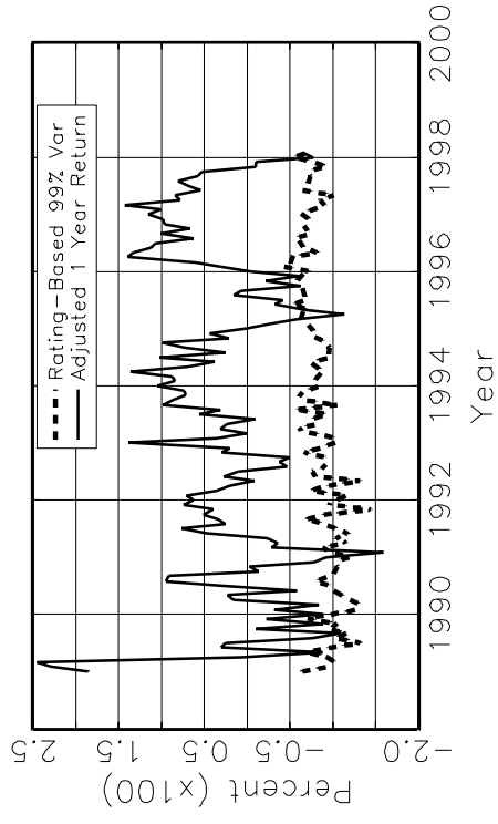
Quartile Portfolio 2
