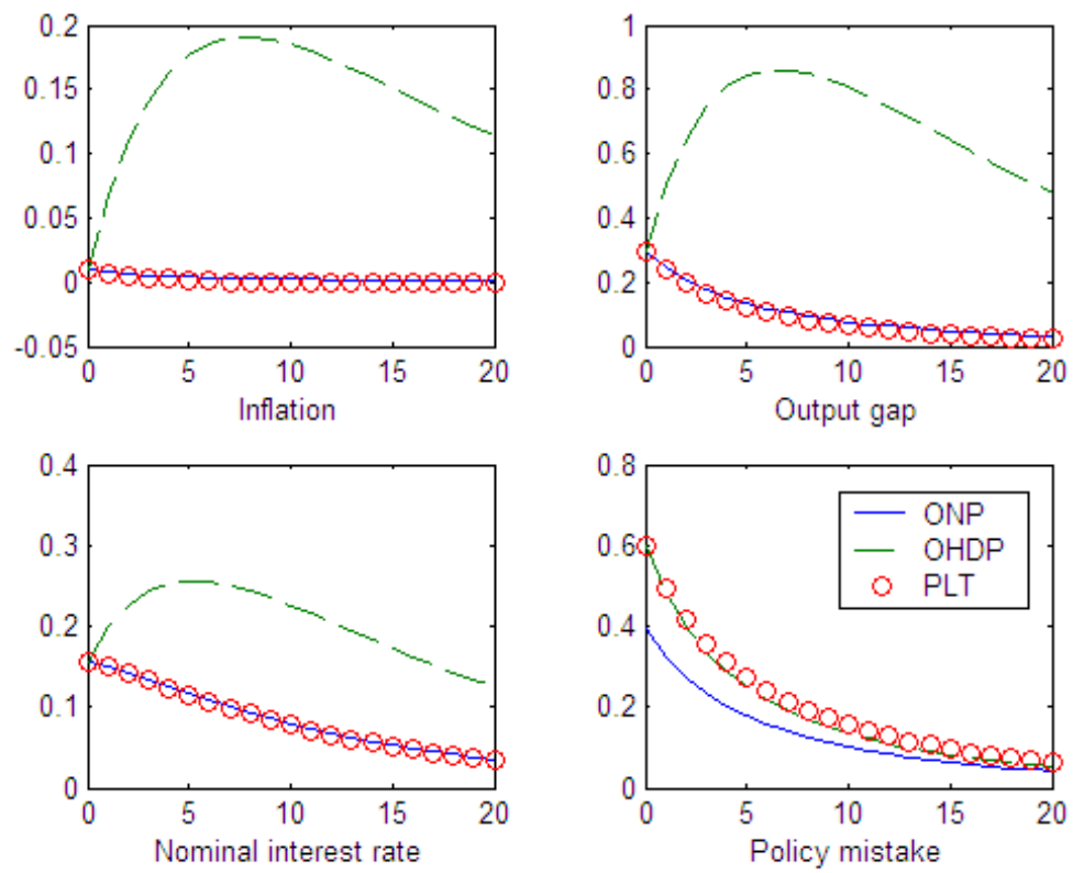
Chart 2: Responses to a demand shock (benchmark case)
