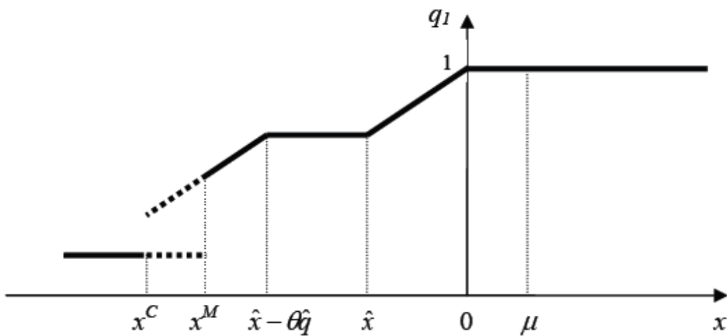
Chart 4: The asset price as a function of the shock
