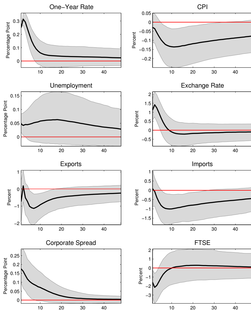
Figure 7 IRFs TO A MONETARY POLICY SHOCK - FULL SPECIFICATION.
